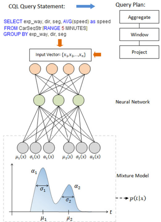
FIGURE 5. Overview of the proposed approach for predicting the resource usage distribution of continuous queries.
