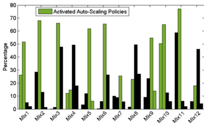
FIGURE 7. The probabilities of the randomly generated auto-scaling policies for 12 (out of 32) mixes of test queries. Each query mix evaluated against four auto-scaling policies as shown in the form of bright and dark coloured bars. The bright and dark bars within each policy set respectively show the activated and not activated rules at run-time. Our technique has successfully characterized the highly possible policies for all mixes but Mix 4, 8, and 12.
