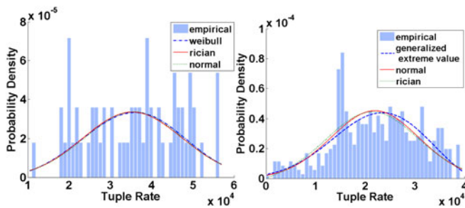
FIGURE 8. Best fit of sent tuple per second against different distribution models. The figures contain probability density of average tuple sent per second for the speed rate of (a) 50 K and (b) 100 K for two different queries.
