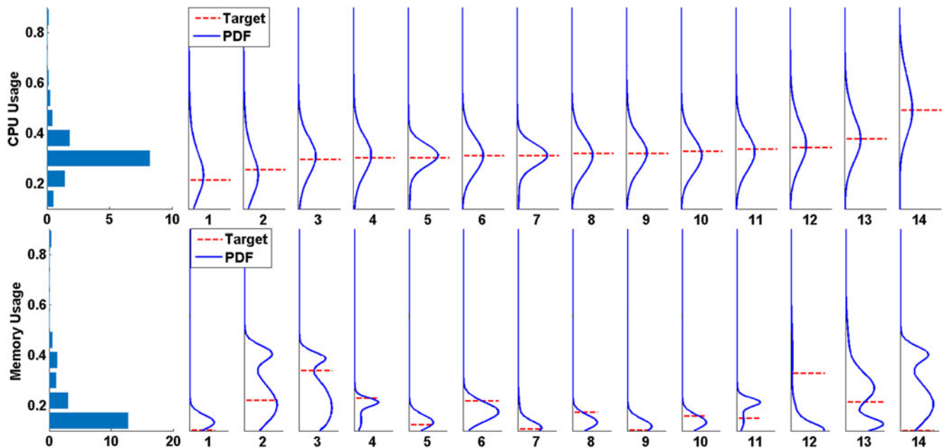
FIGURE 10. Sample PDF predictions for (a) CPU and (b) memory usage from TPC-H workload.
