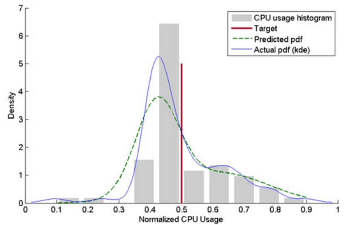
FIGURE 2. Sample distribution prediction of CPU usage for Neg-AccTollStr query. Actual PDF is a fitted KDE function against the actual CPU usage which is used for clarity and comparison with the prediction.
