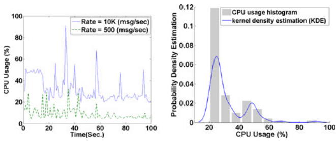
FIGURE 1. (a) CPU usage of the query against 500 and 10 K tuple/sec arrival rates. (b) Normalized histogram and KDE fitted to CPU usage of CurActiveCars query against 10 K data arrival rate.
