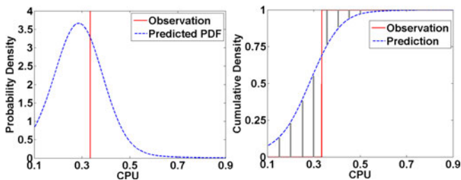
FIGURE 9. (a) predicted PDF and the observation (b) schematic sketch of the CRPS as the difference between CDFs of prediction and observation.
