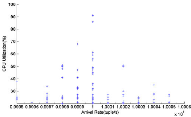
FIGURE 4. CPU usage of CurActiveCars query against average arrival rates showing the multi-valued mapping situation from the same input.
