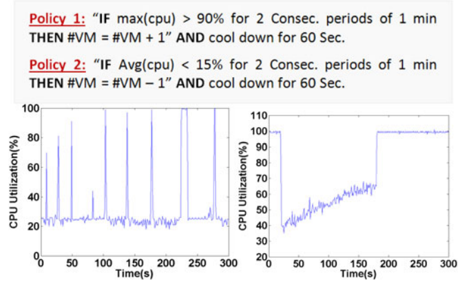
FIGURE 6 The CPU utilization of (a) NegAccTollStr and (b) Seg-Toll queries for 5 minutes. The sample auto-scaling policies cause oscillation behaviour in NegAccTollStr workload, since they have been defined irrespective of the workload CPU usage distribution.
