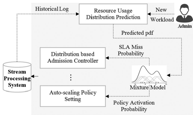
FIGURE 3. Our approach builds an MDN model based on the historical logs of queries to predict distribution of new incoming workloads. The predicted PDFs are then used for developing two novel workload management strategies: a) Distribution based admission control, and b) Auto-scaling policy setting.
